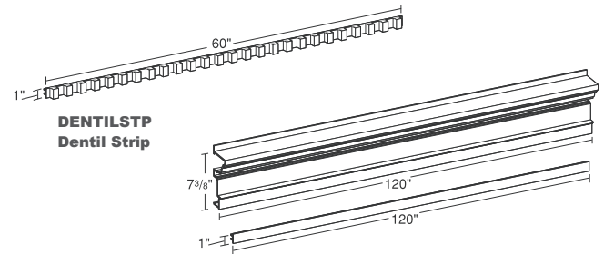
MANTEL 120 Mantel System with Plain Cover Strip
