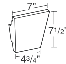
KEYSTN Keystone for Mantel system
